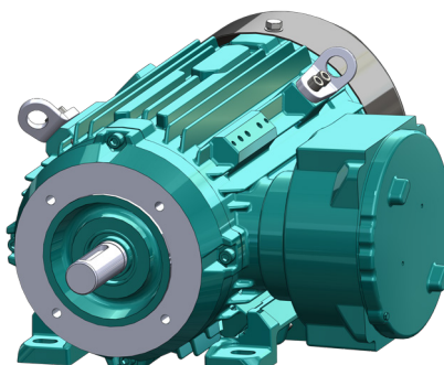
B34 [Terminal box right]
